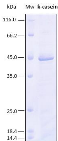
Figure 1. SDS-PAGE analysis (15%) of 6 \mu l of the recombinant allergen \kappa -casein. Purity is approx. 90% as determined by gel electrophoresis.
