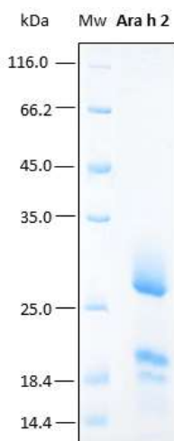
Figure 1. SDS-PAGE analysis (15%) of 5 \mu l of the recombinant allergen. Purity is >95% as determined by gel electrophoresis. Both bands represent the complete protein, with the higher band containing one O-glycosylation, as determined by MALDI-TOF analysis.
