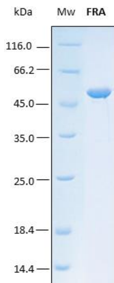
Figure 1. SDS-PAGE analysis (12%) of 1 µl of recombinant FRA. Purity is > 98% as determined by gel electrophoresis.
