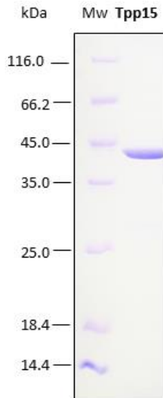
Figure 1. SDS-PAGE analysis (15%) of 3 µl of recombinant Tpp15. Purity is > 98% as determined by gel electrophoresis.
