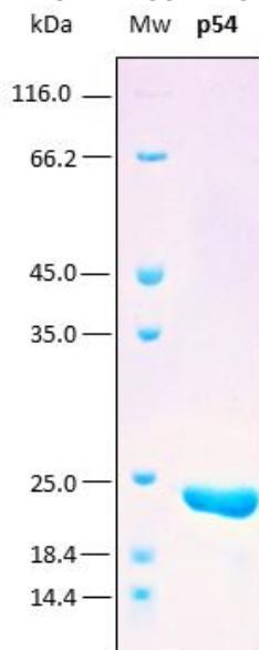
Figure 1. SDS-PAGE analysis (15%) of 2 µl of recombinant p54. Purity is > 95% as determined by gel electrophoresis.
