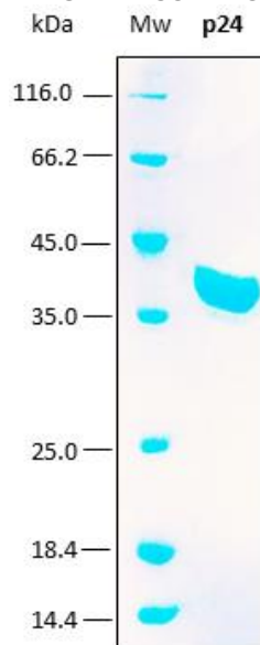
Figure 1. SDS-PAGE analysis (15%) of 3 \mu l of recombinant p24. Purity is >98% as determined by gel electrophoresis.
