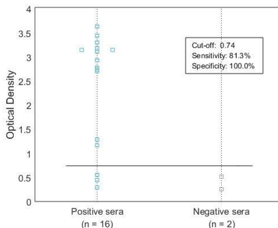
Figure 2. The dot plot graph illustrates the distribution of positive and negative sera by an indirect IgG ELISA with a p24 plate coating of 1 \mu g/ml. Pre-validated sera by Dx (Izasa) were used in this analysis. The chart shows the optical density at 450/620 nm for positive (blue) and negative (grey) IgG sera.
