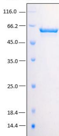
Figure 1. SDS-PAGE analysis (15%) of 3 µl of recombinant ChimChagas1. Purity is > 98% as determined by gel electrophoresis.
