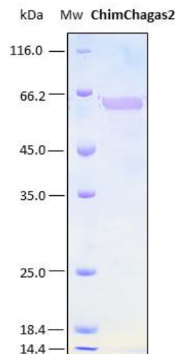
Figure 1. SDS-PAGE analysis (12%) of 2 \mu l of recombinant ChimChagas2. Purity is > 98% as determined by gel electrophoresis. Bands which are slightly smaller correspond to this same protein as it is showed in a western blot performed with a his-tag monoclonal antibody
